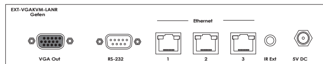
EXT-VGAKVM-LANRX (受信機)
