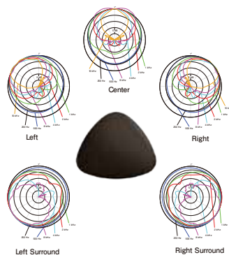
Polar patterns Typical directional characteristics of DPA 900 (normalized)
