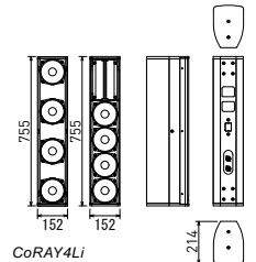
CoRAY4Li
